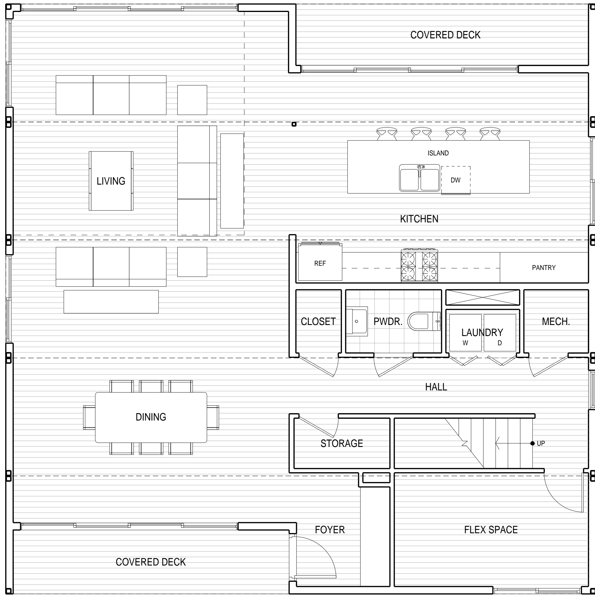
FIRST FLOOR
